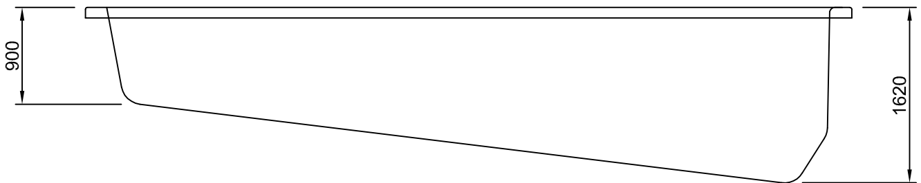
ELEVATION PEGASUS SWIMMING POOL
