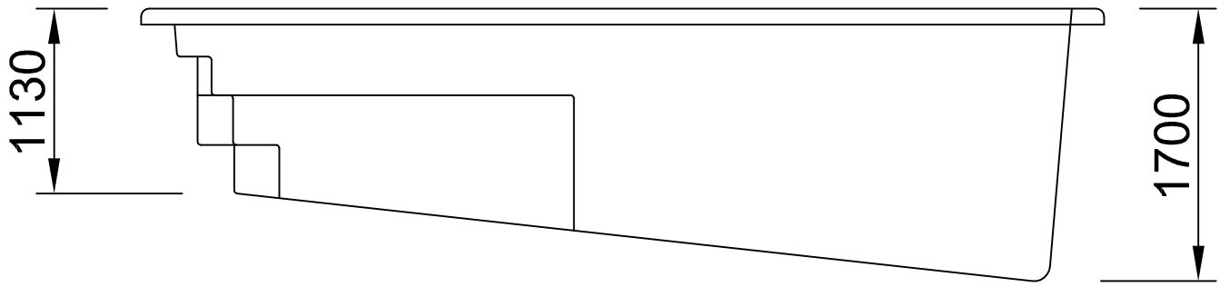
ELEVATION WEST AUSSIE SWIMMING POOL
